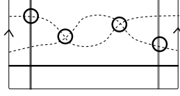
FIGURE 1. The quadrangle, whose vertical sides are identified accordingly with the arrows and horizontal sides represent the vertex V , is Q(\mathbb{R}) . The cubic section S(\mathbb{R}) is in thick black, while C_{ijk}(\mathbb{R}) and C_{jkt}(\mathbb{R}) in dashed. The generatrices L_i(\mathbb{R}) and L_t(\mathbb{R}) are in grey.
